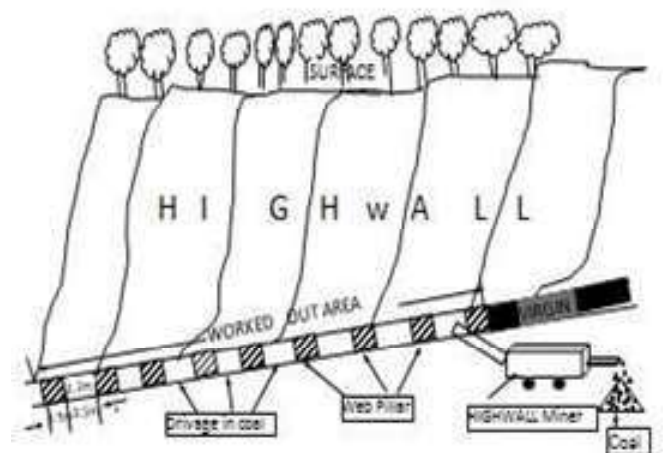
Fig. 3: High Wall Mining Layout in Extraction of Thin Seam
