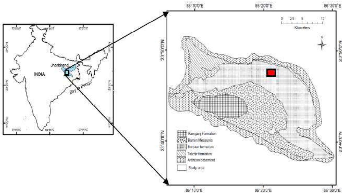
Fig. 1: Location map of study area along generalized geological map of Jharia coalfield
